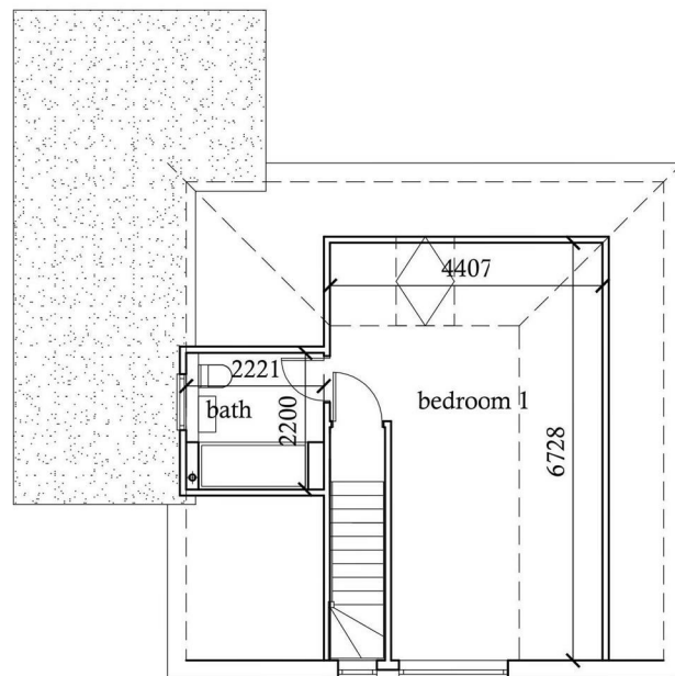
PROPOSED FIRST FLOOR PLAN 1:100
